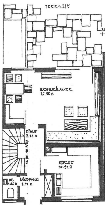
Grundriss, EG:
